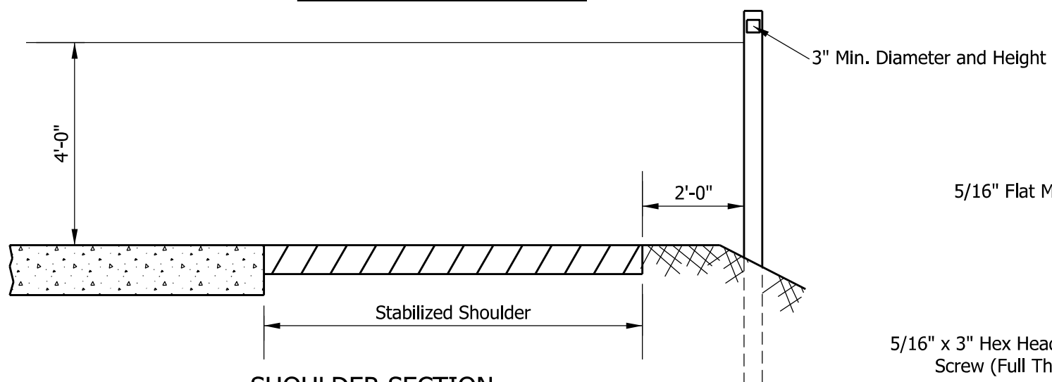
SHOULDER SECTION
