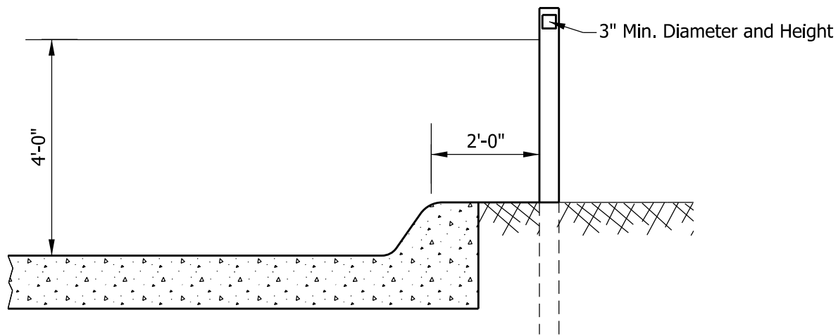
CURB SECTION
